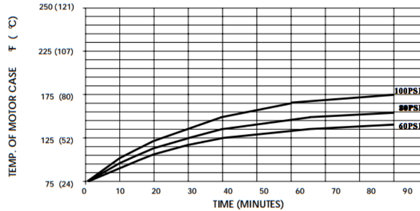
THIS GRAPH IS FOR USE AS A DESIGN GUIDE. IT IS BASED ON RUNNING CONTINUOUSLY WITH AN AMBIENT TEMPERATURE OF 70° F IN STILL AIR.
